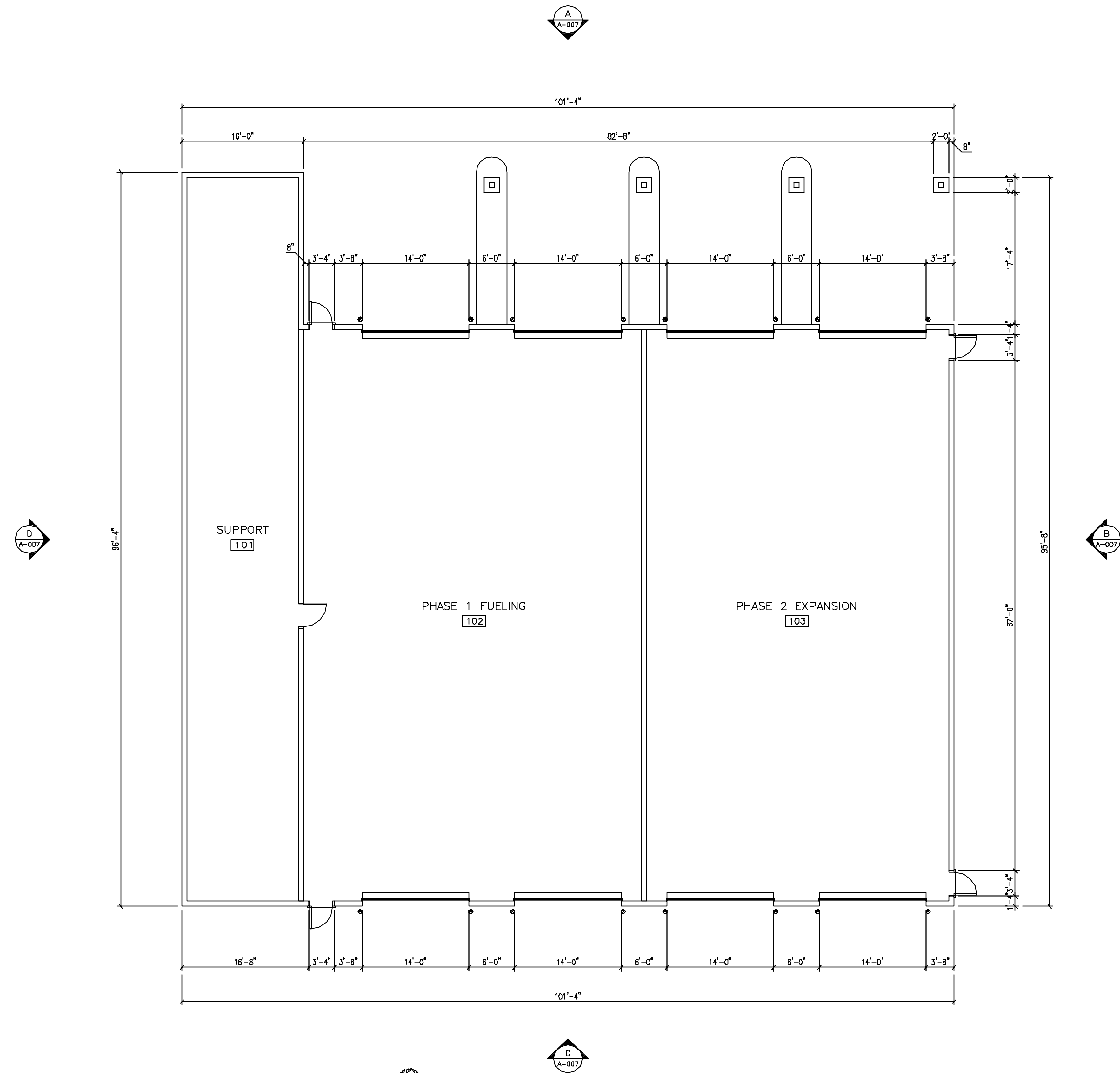
FLOOR PLAN 1/8" = 1'-0"
