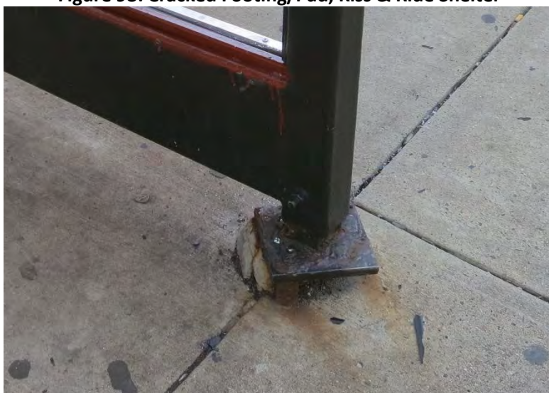
Figure 98: Cracked Footing/Pad, Kiss & Ride Shelter
