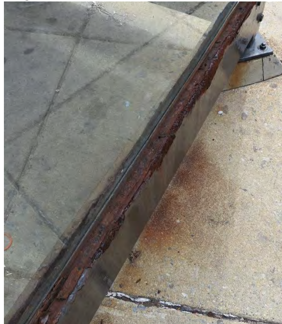
Figure 107: Poor Frame Condition, Shelter F
