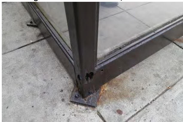
Figure 130: Hole in Frame, Shelter C
