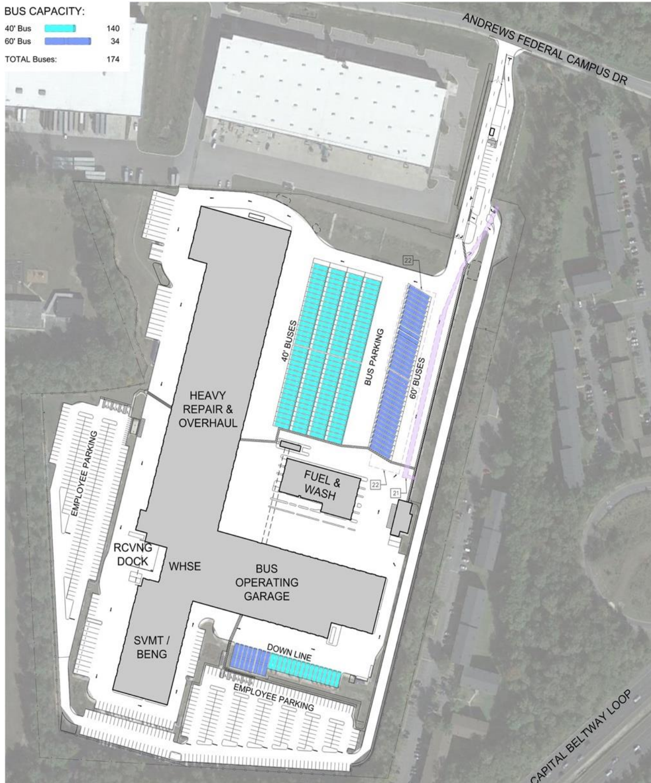
Figure 4-3. Andrews Federal Center Garage – Existing Site Layout
