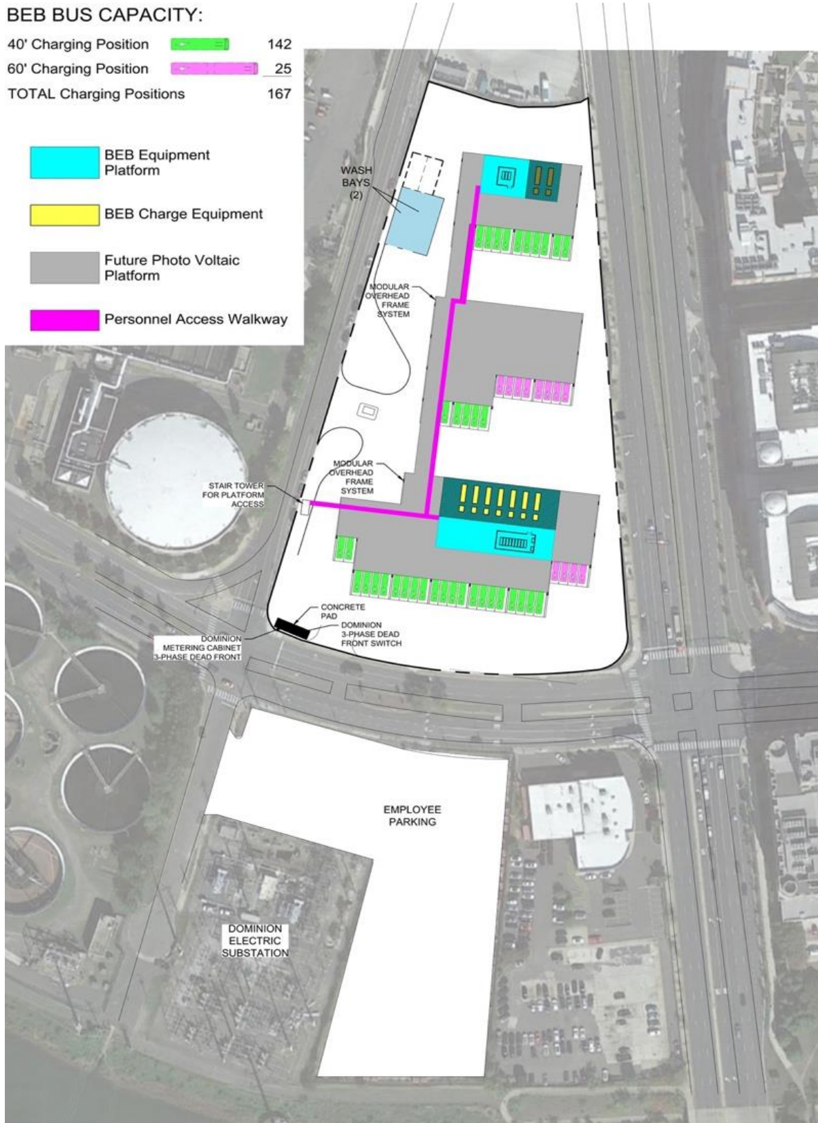
Figure 4-14. Four Mile Run Garage – Proposed Site Layout
