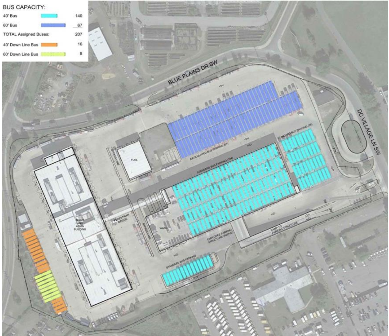
Figure 4-25. Shepherd Parkway Garage – Existing Site Layout
