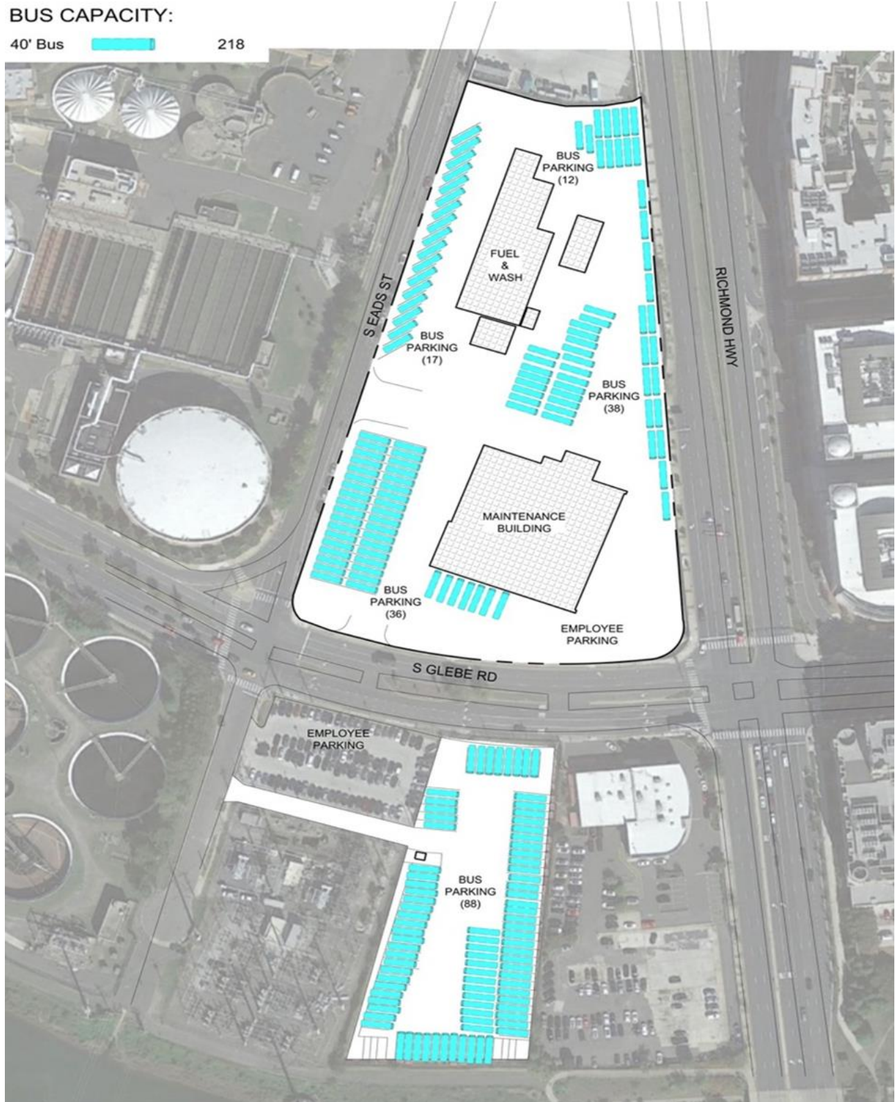
Figure 4-13. Four Mile Run Garage – Existing Site Layout
