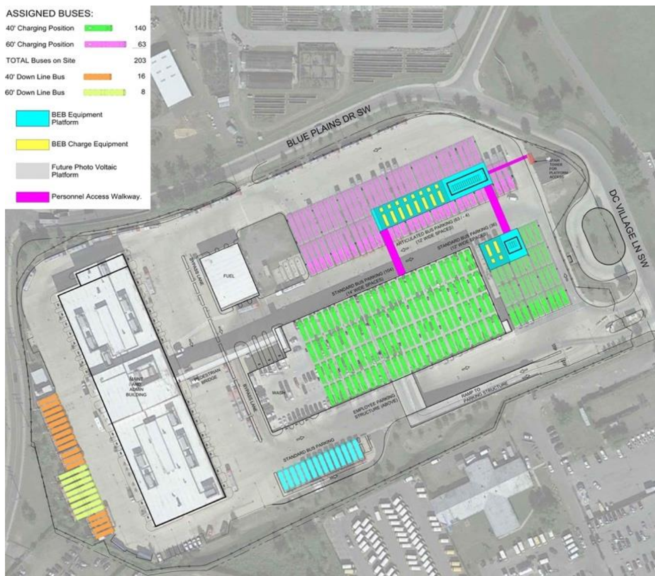
Figure 4-26. Shepherd Parkway Garage – Proposed Site Layout
