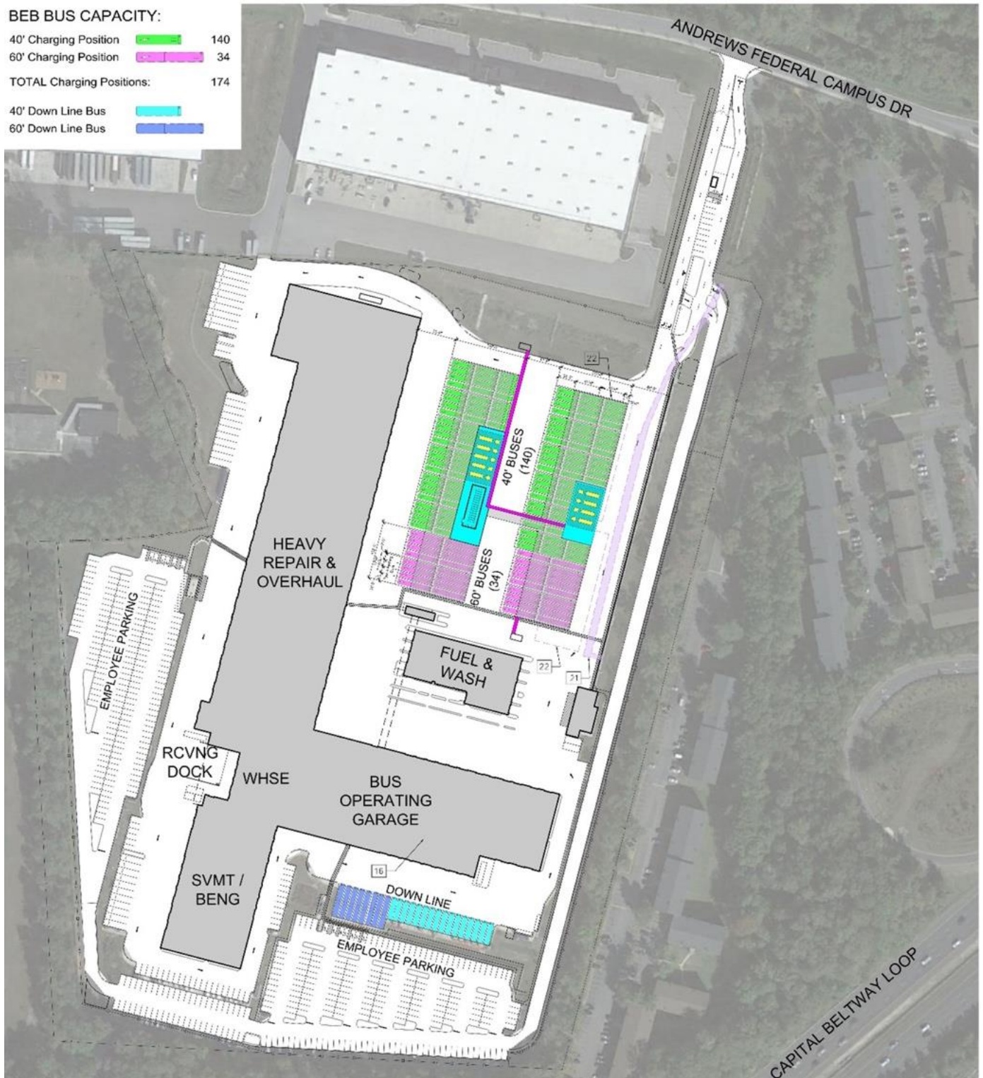
Figure 4-4. Andrews Federal Center Garage – Proposed Site Layout
