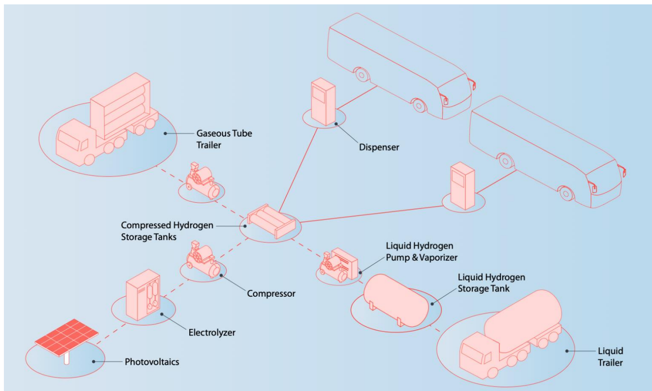
Figure 2-8. Typical Fuel Cell Electric Bus System
