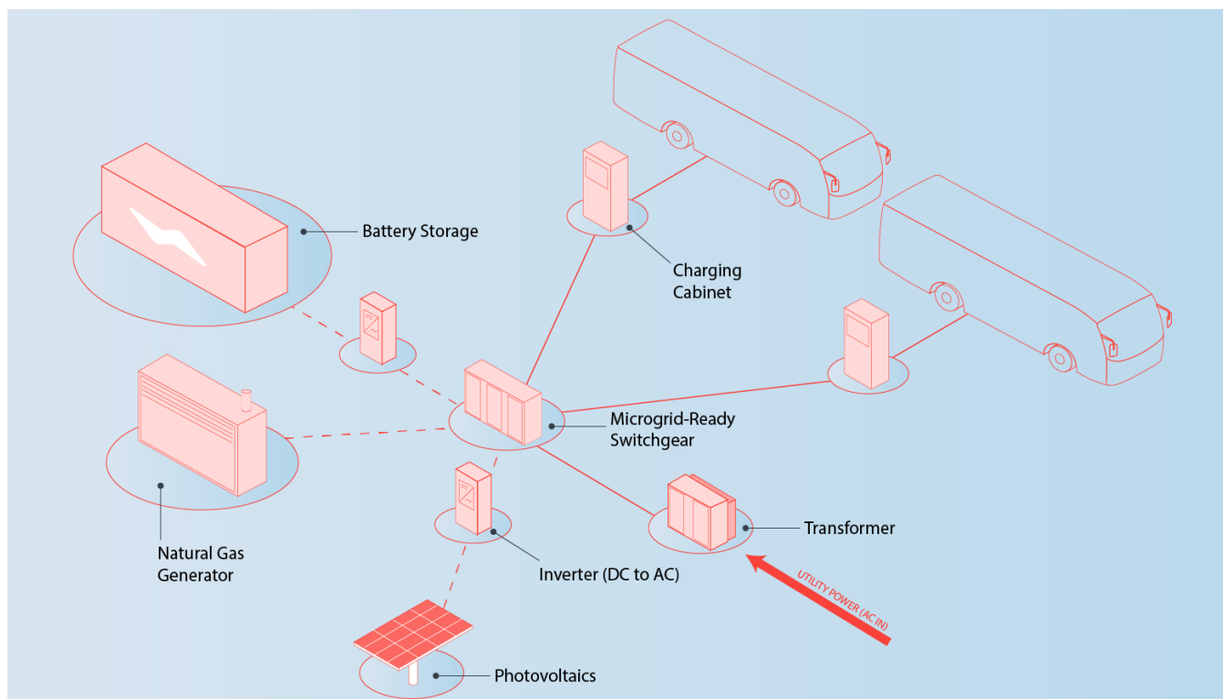
Figure 2-7. Typical Battery-Electric Bus System
