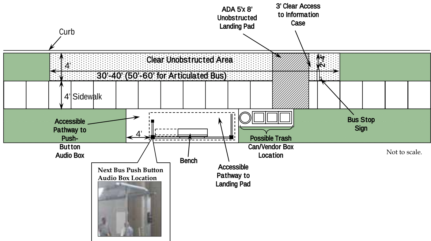
Figure 3-20: Enhanced Service Bus Stop
