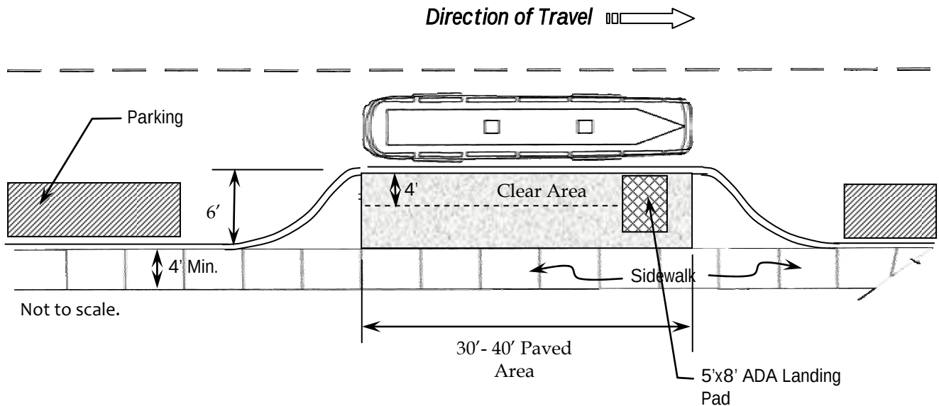
Figure 2-7: Curb Bulb
