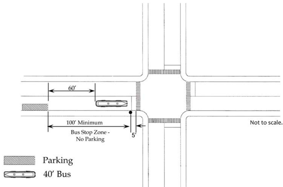
Figure 1: Typical Near-Side Bus Stop Location
