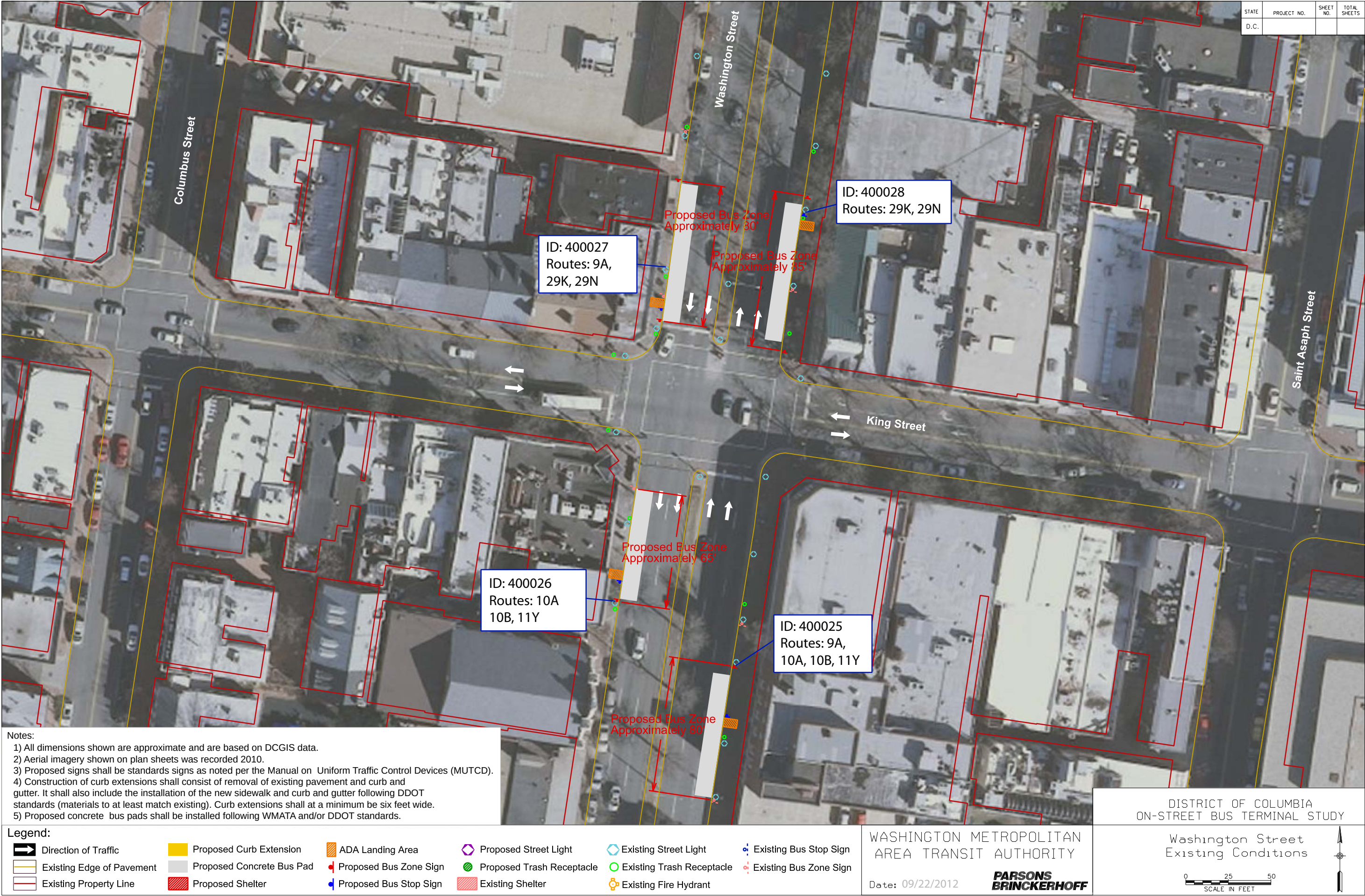
Figure 99 Foldout – Recommendations Plan View – Washington Street and King Street
