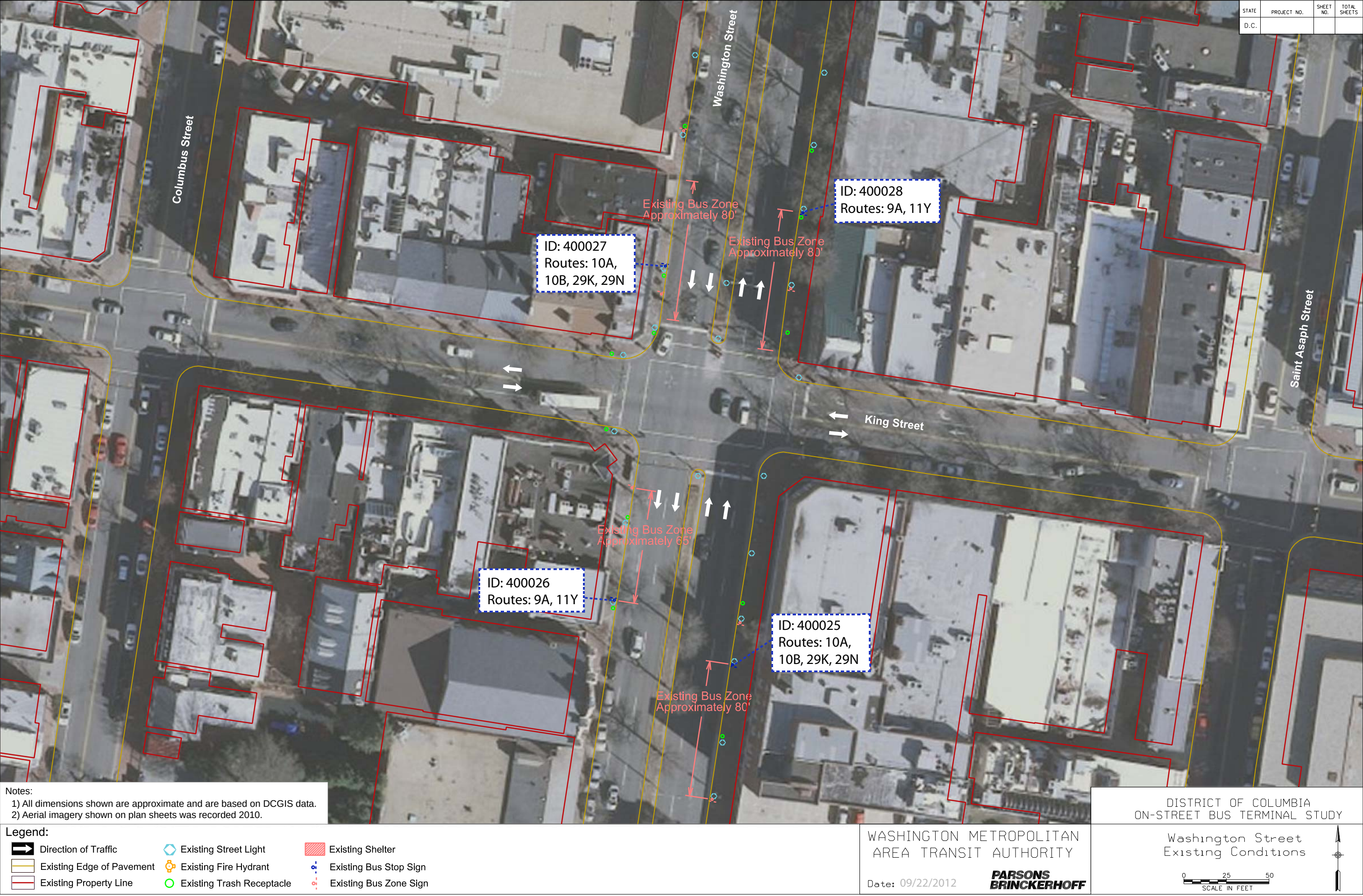
Figure 76: Foldout – Existing Conditions Plan View – Washington Street at King Street
