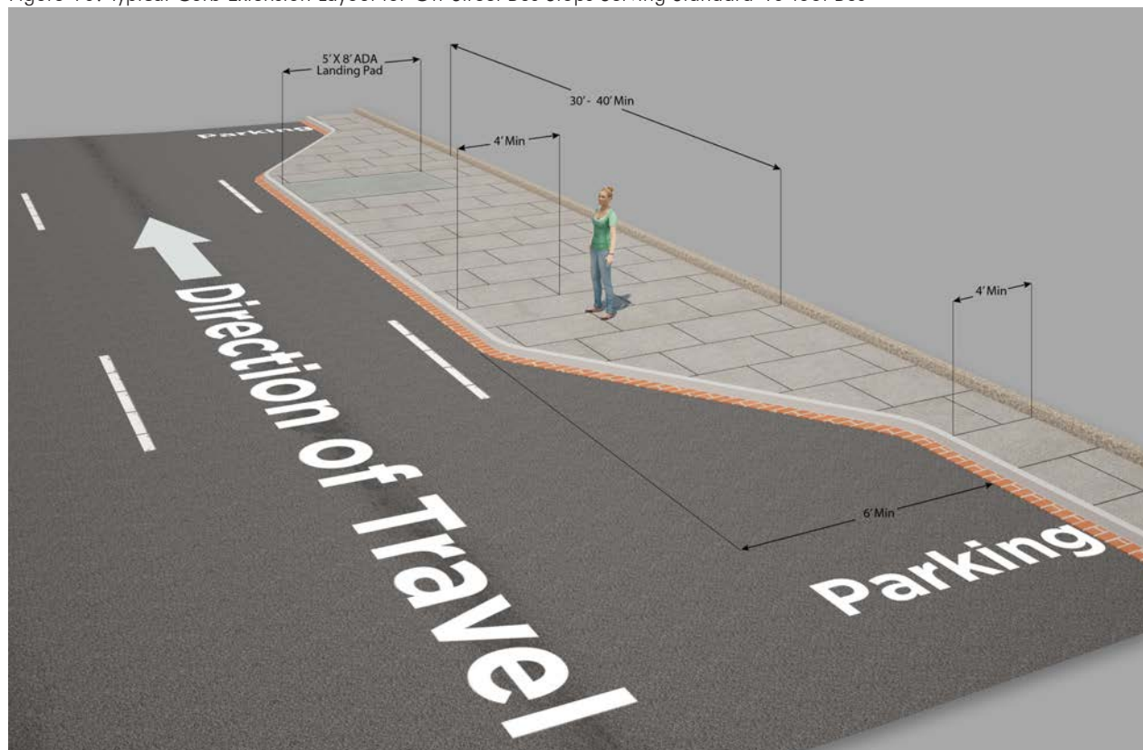
Figure 10: Typical Curb Extension Layout for On-Street Bus Stops Serving Standard 40-foot Bus
