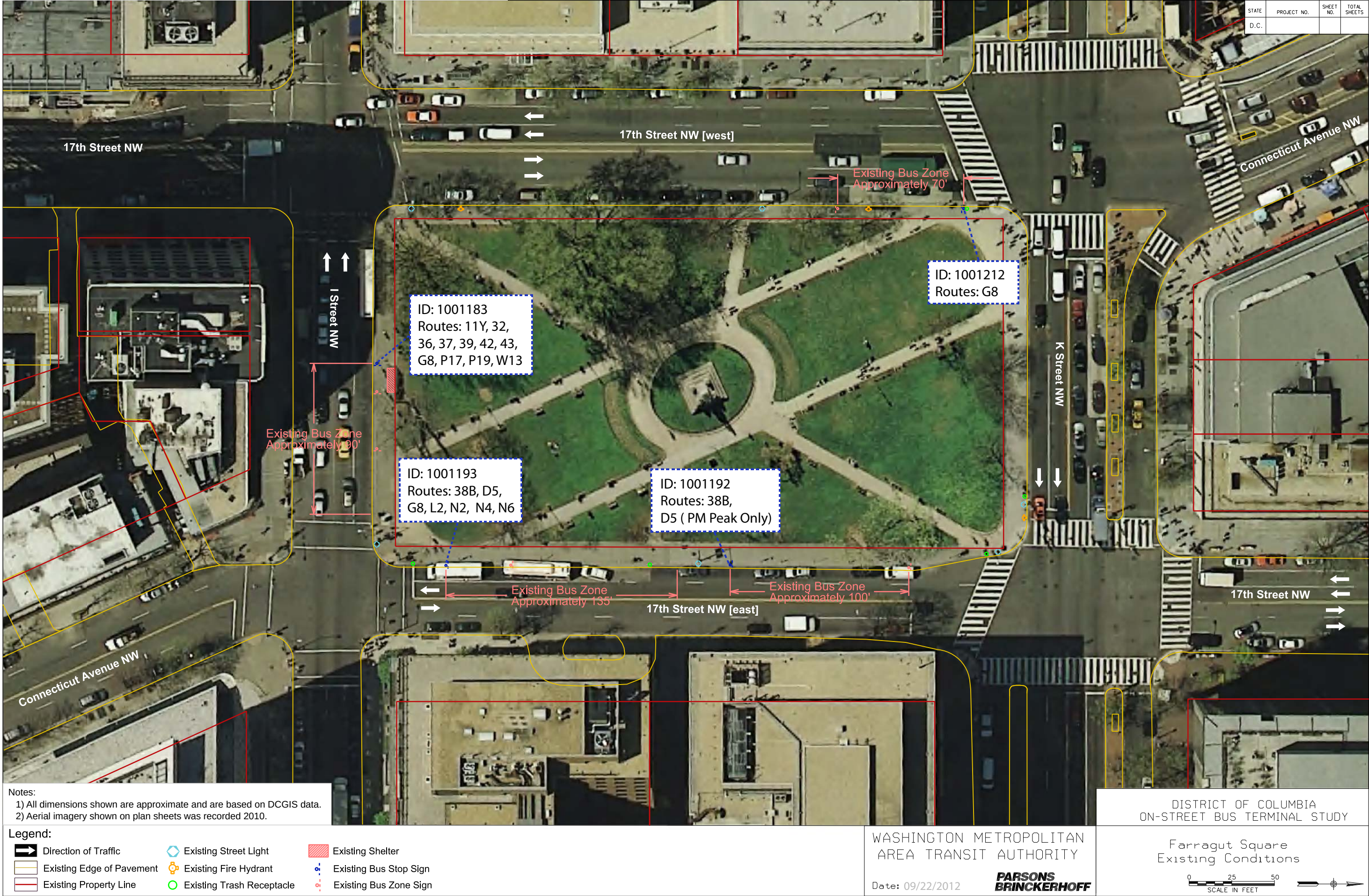
Figure 45: Foldout – Existing Conditions Plan View – Farragut Square
