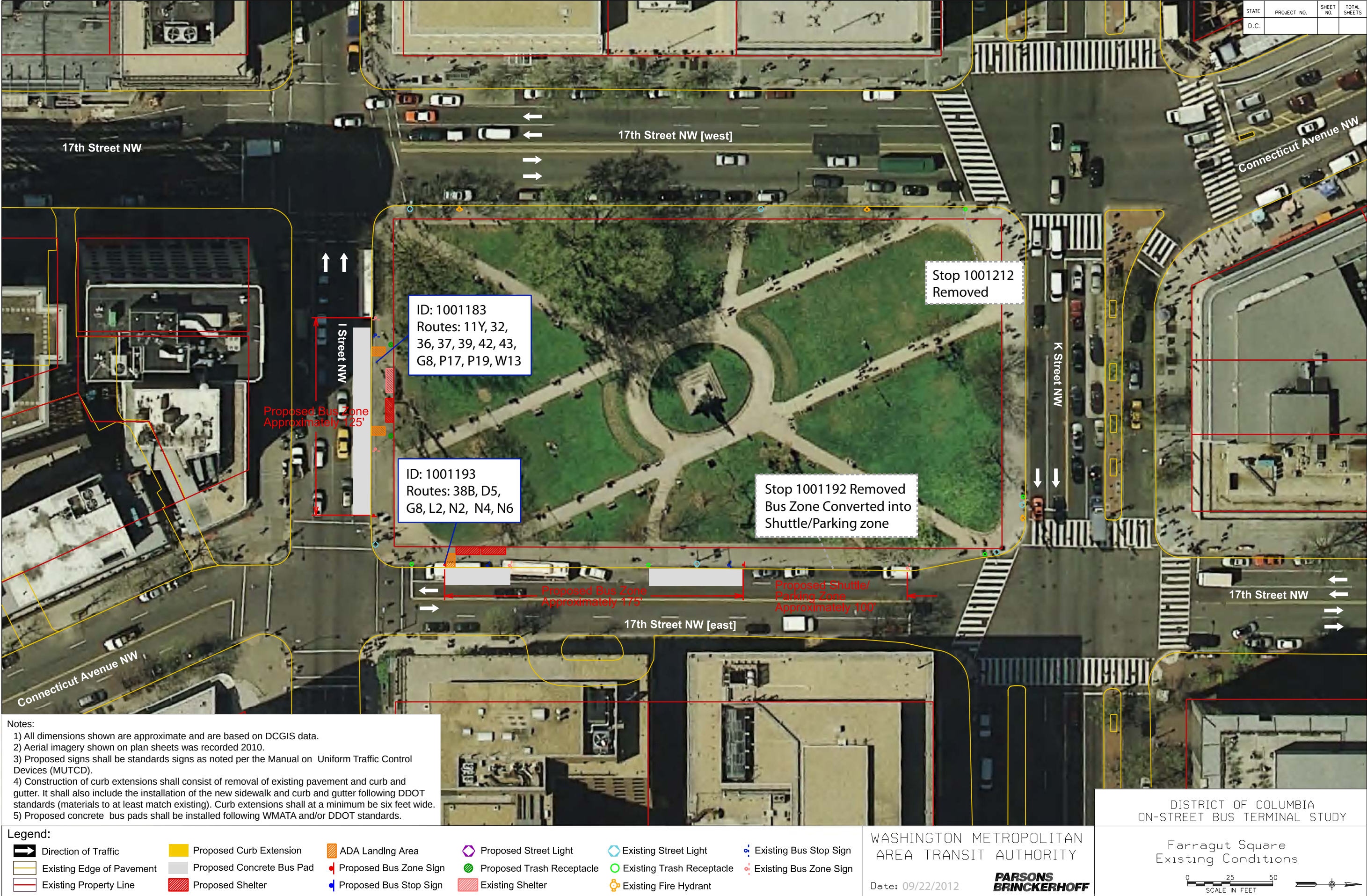
Figure 82: Foldout – Recommendations Plan View – Farragut Square
