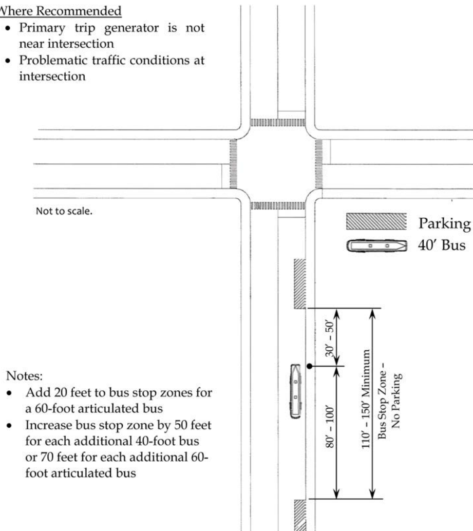
Figure 3: Typical Mid-Block Bus Stop Location
