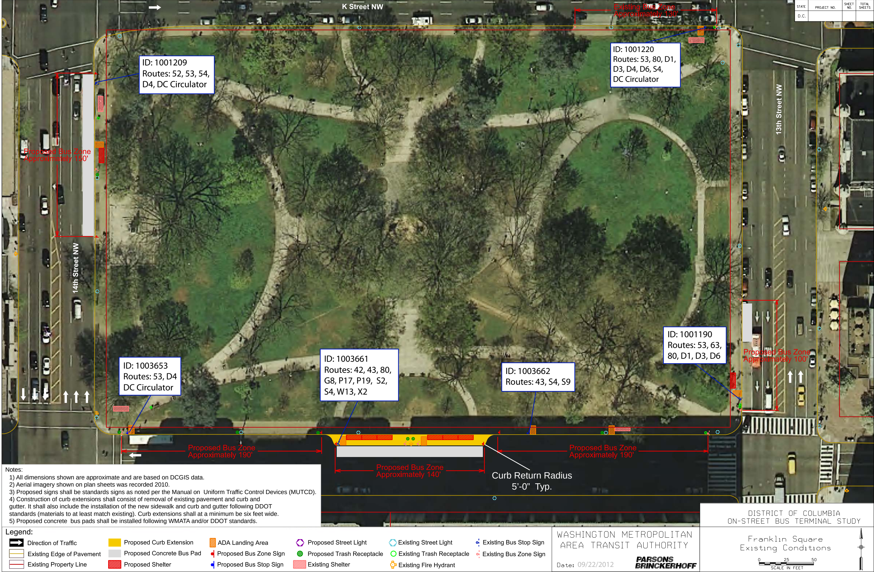
Figure 86 Foldout – Recommendations Plan View – Franklin Square
