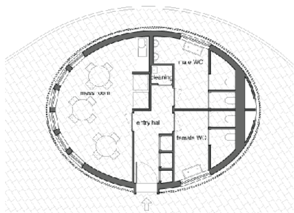
Daggenham Bus Facility Hub Floor Plan
