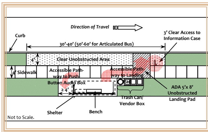
Figure 27. Enhanced Service Stop with Shelter
