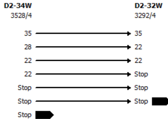
Figure 13 – Example of Site-Specific Simulation Signal Control Lines
