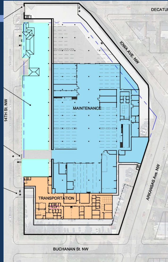
Intermediate Level
