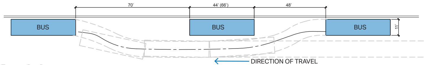
Figure 3.1 —Illustrations depicting dimensions and alignment of typical bus bays.
