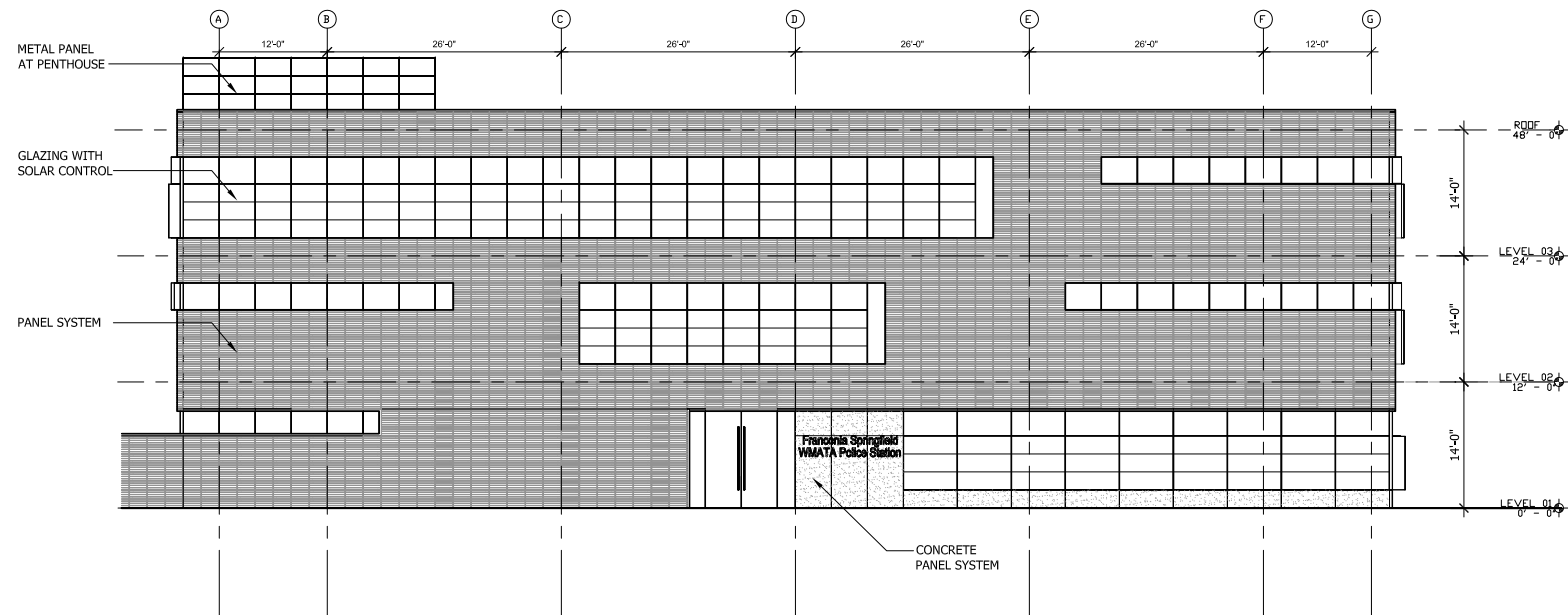
3 SOUTH ELEVATION
