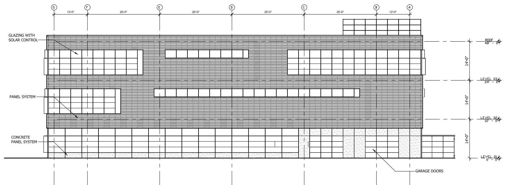
1 NORTH ELEVATION
