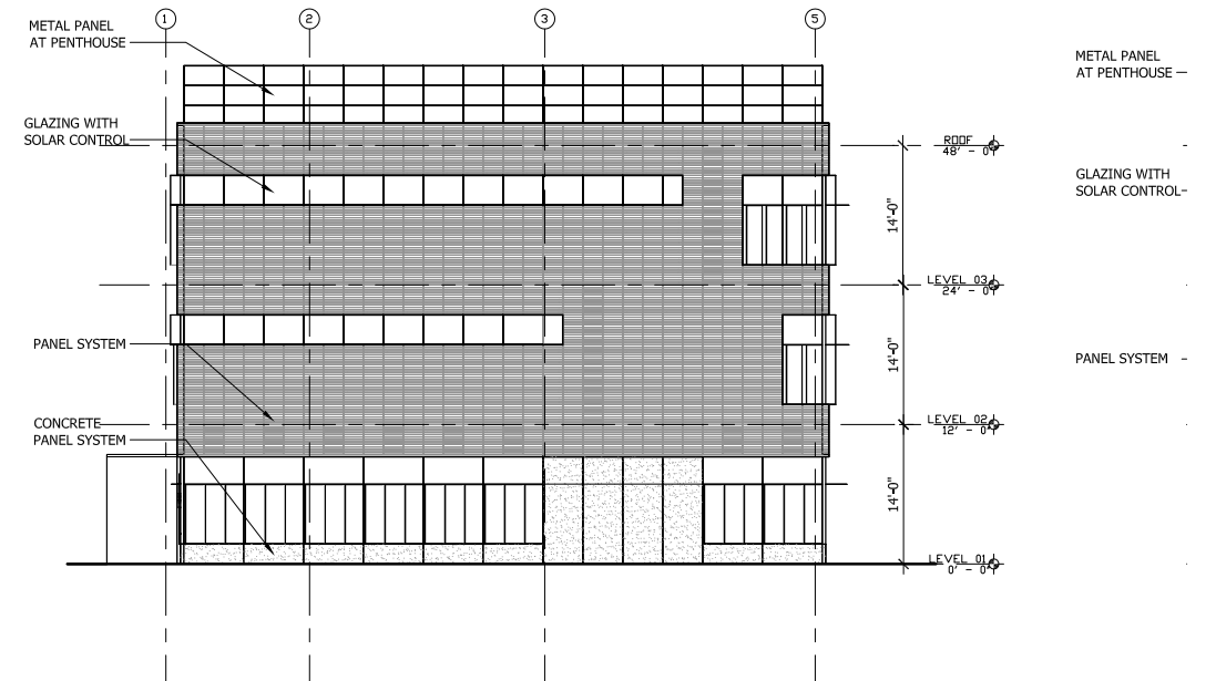
2 EAST ELEVATION
