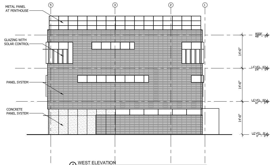
4 WEST ELEVATION
