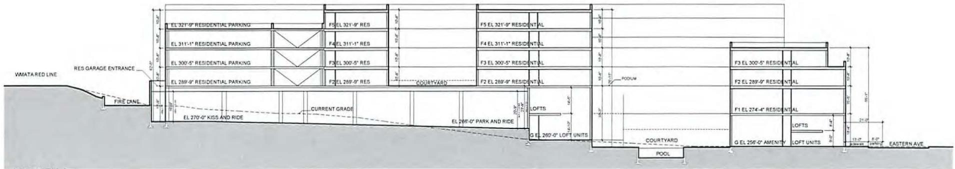
SECTION A
