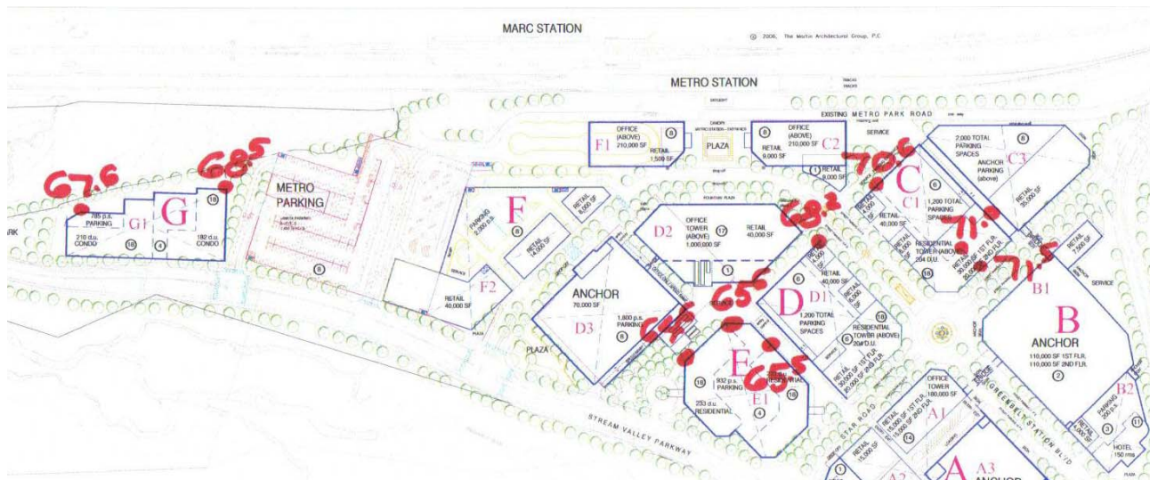
Figure 9. Combined DNL 185 Feet Above Ground in the Absence of Buildings
