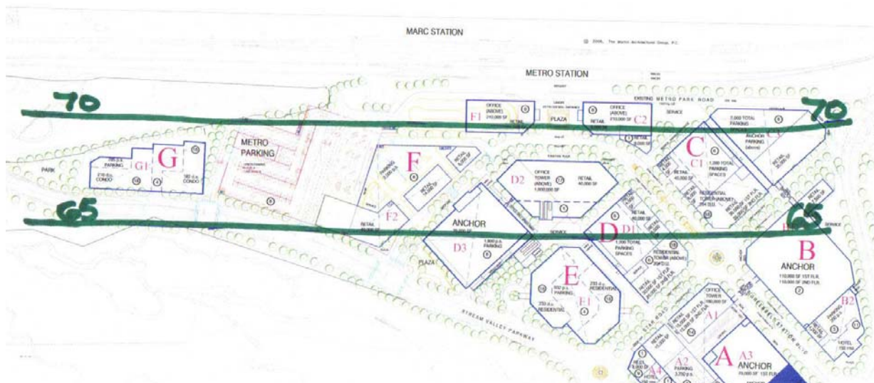
Figure 8. Railroad DNL at Facades of Residences on 18 th Floor in the Absence of Buildings
