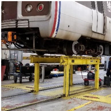
Lifts with Body Jacks Collapsed
