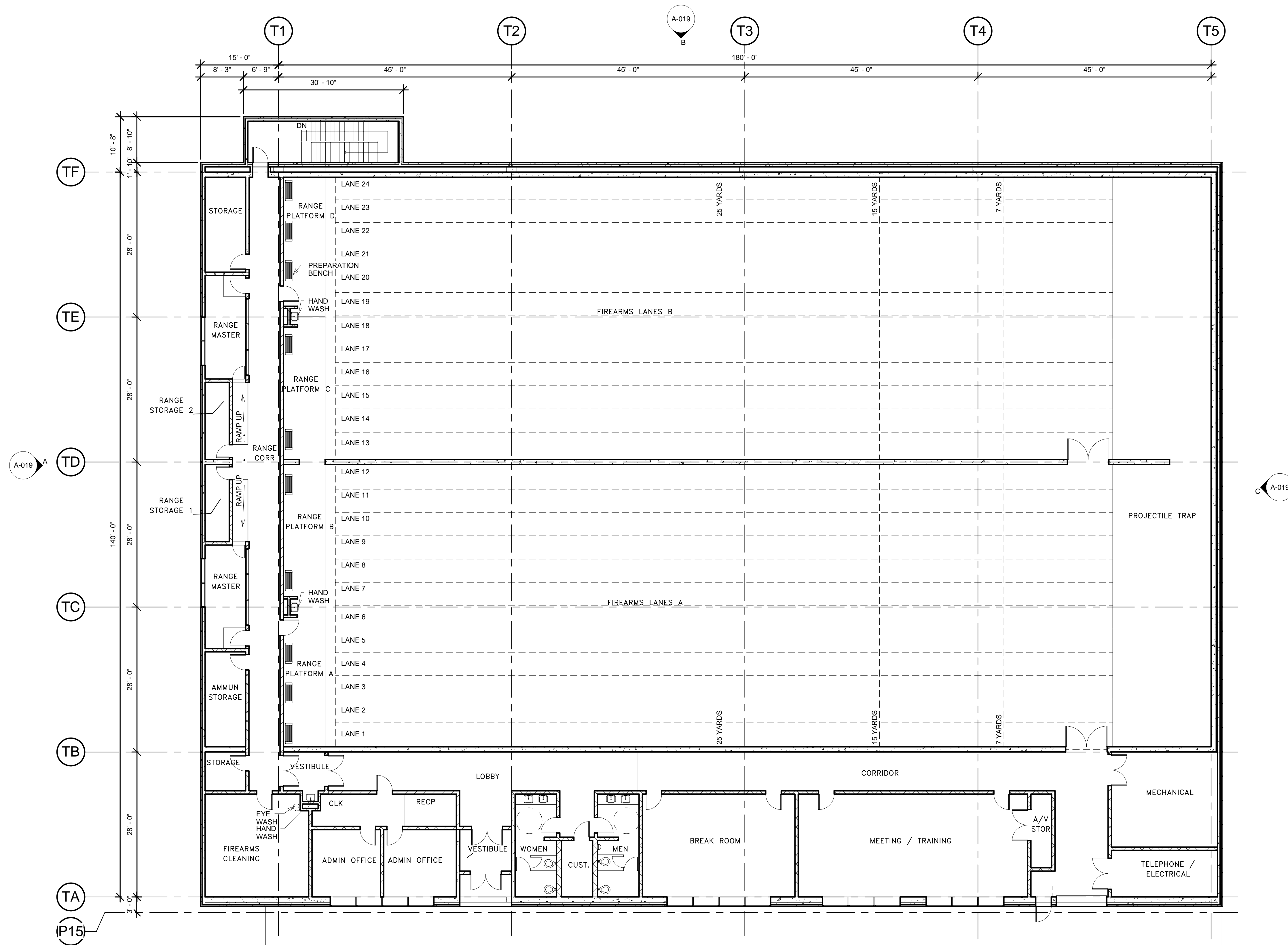
A SECOND FLOOR PLAN 3/32" = 1'-0"
